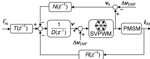
Fig. 8 Block diagram of the current controller including the anti-windup strategy
