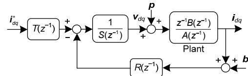
Fig. 7 Block diagram of the current loop with the directly designed two-degree-of-freedom (2DOF) discrete-time controller
