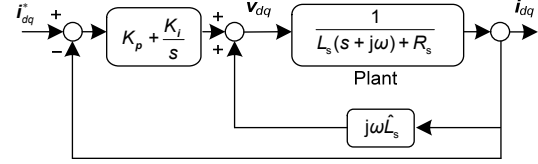
Fig. 4 Block diagram of the current loop with the continuous-time state feedback PI controller
